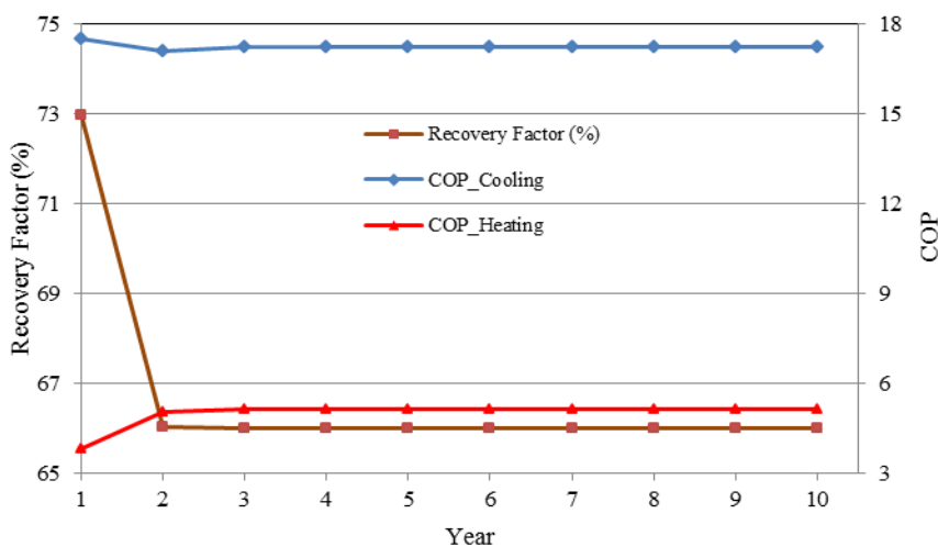
Fig.7. The Recovery Factor of the Aquifer and COP in the ATES Coupled with a Heat Pump, for Ten Years of Operation
