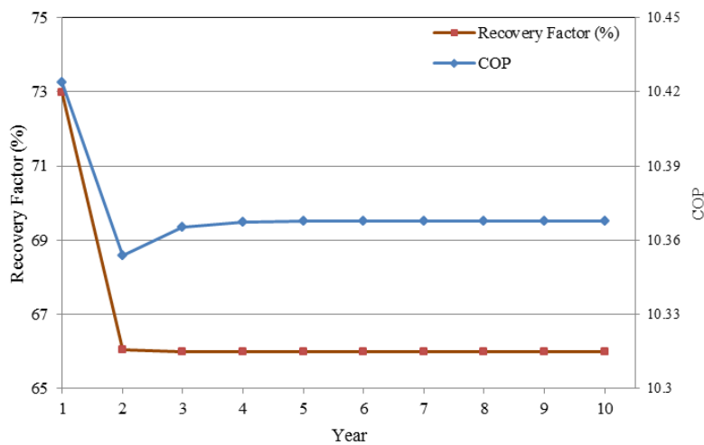
Fig.6. The recovery factor of the aquifer and COP at the period of ten years
