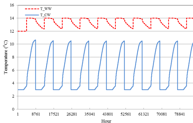
Fig. 5. Temperature variation of cold and warm wells at ten years operation
