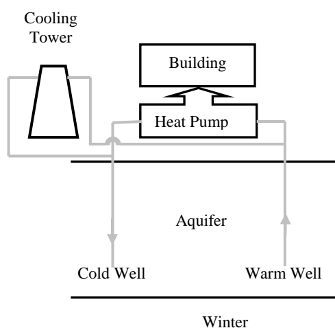
Fig. 2. Combination of ATES with a heat pump for heating and cooling of the buildings
