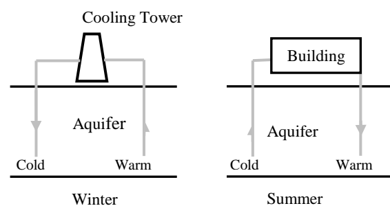
Fig. 1. Cooling through ATES alone
