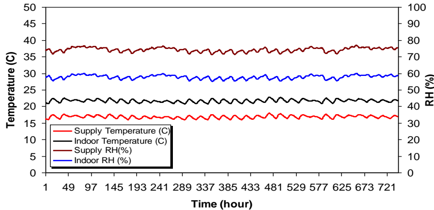
Fig. 5. Simulation responses for the two-row configuration at 6 °C chilled water temperature
