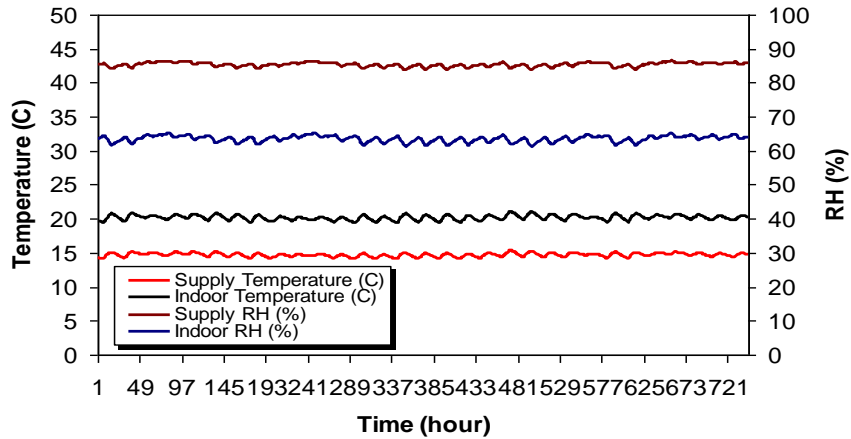
Fig. 4. Simulation responses for the HVAC system
